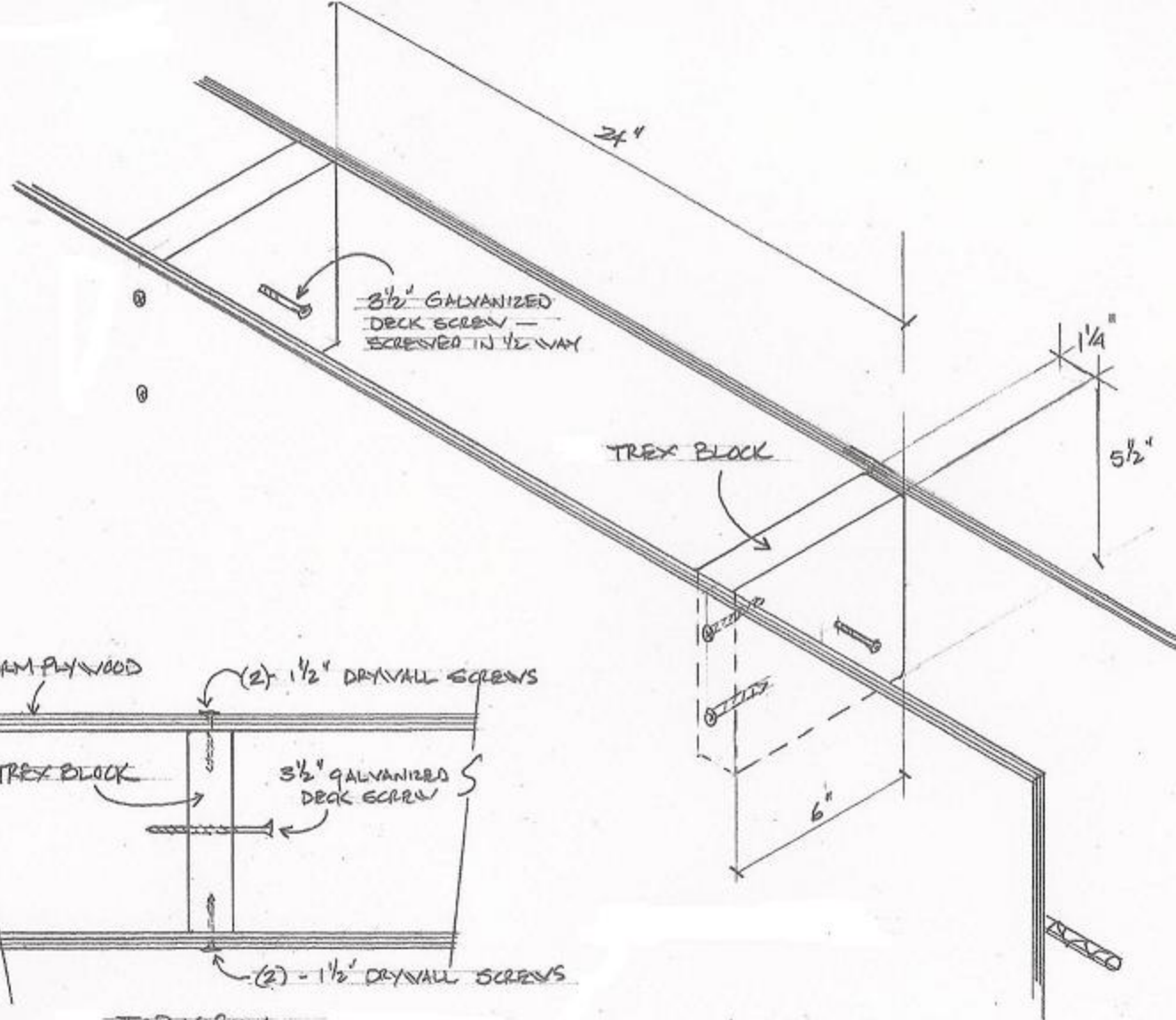
TOP VIEW
